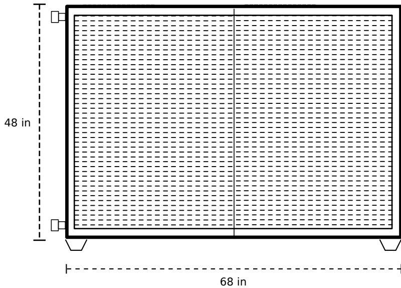
END VIEW
